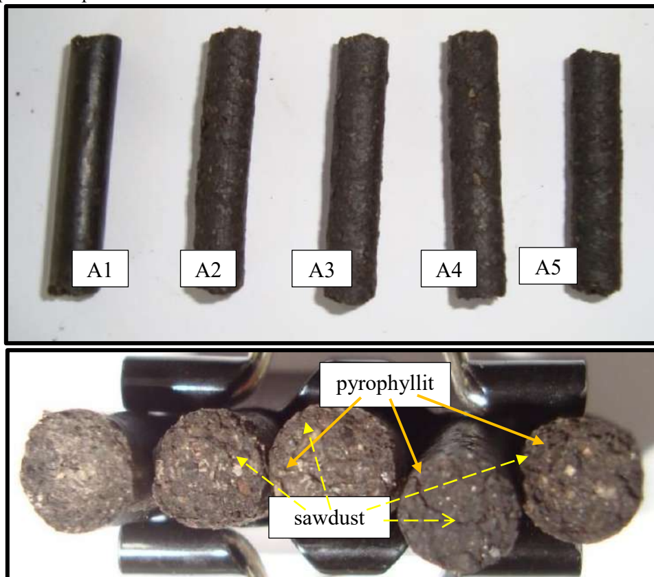
Figure 1. Structural appearance of the briquette and its cross-section
