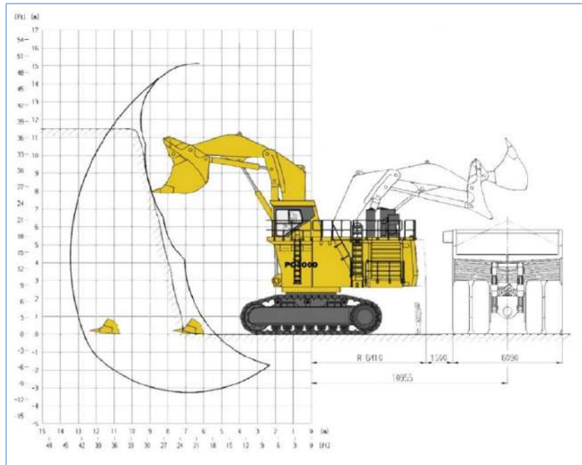
Figure 4. Hydraulic excavator performances for a bench height of 11.5\text{ m} and the associated truck capacity of 165\text{ t}
