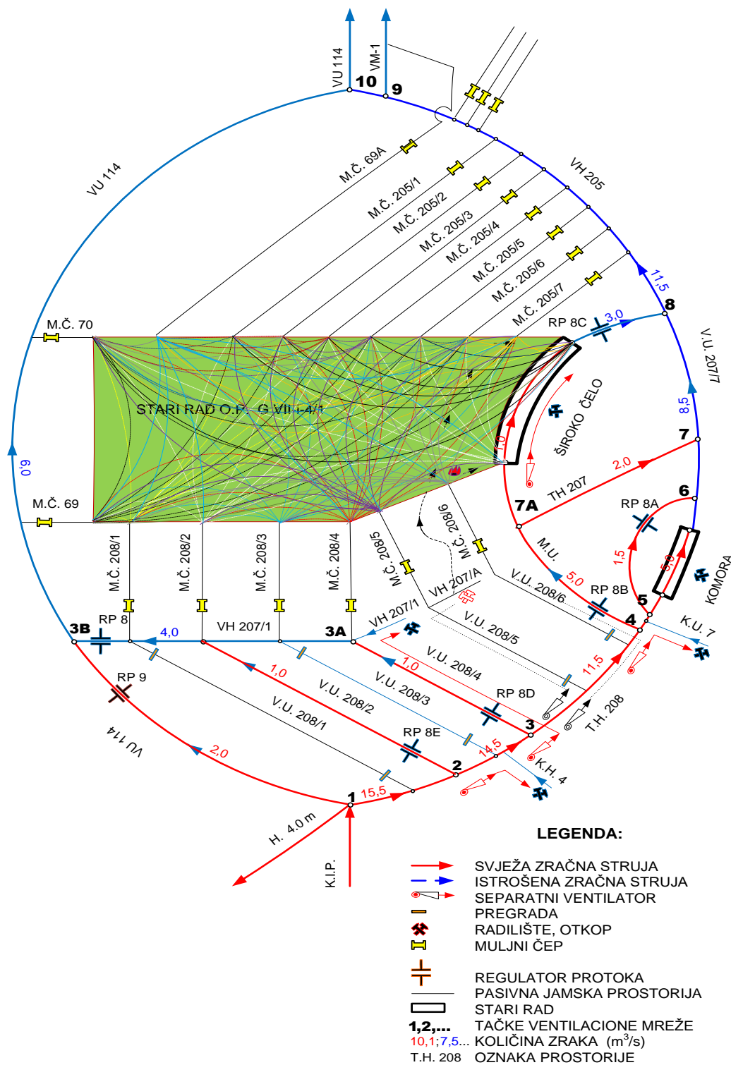
Figure 6. Canonic ventilation scheme of the Eastern part of Raspotočje mine (TB-IV) upon reclosure of the connecting rises VU-208/5 and VU 208/6 and construction of assembly rise (MU); Status on December, 2002 [1] (Graphical analysis of possible air flow lines (migration) through the gob area of longwall face)
