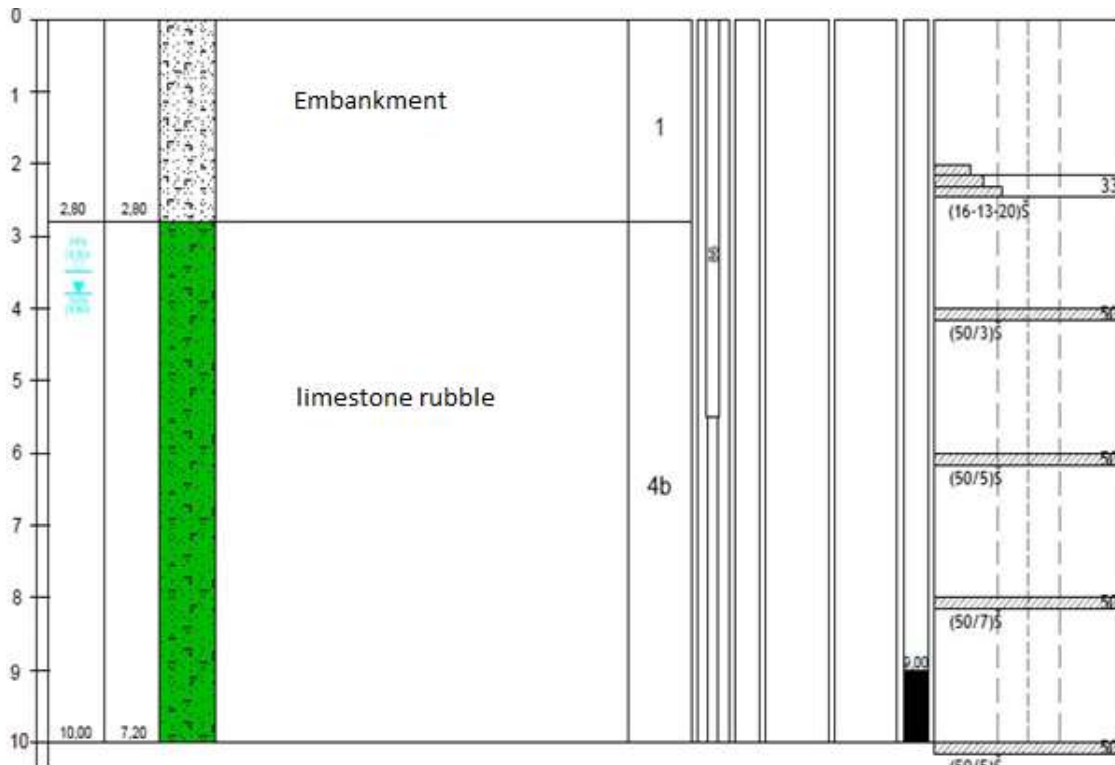
Figure 2. Lithological profile of the BZ - 16 well
