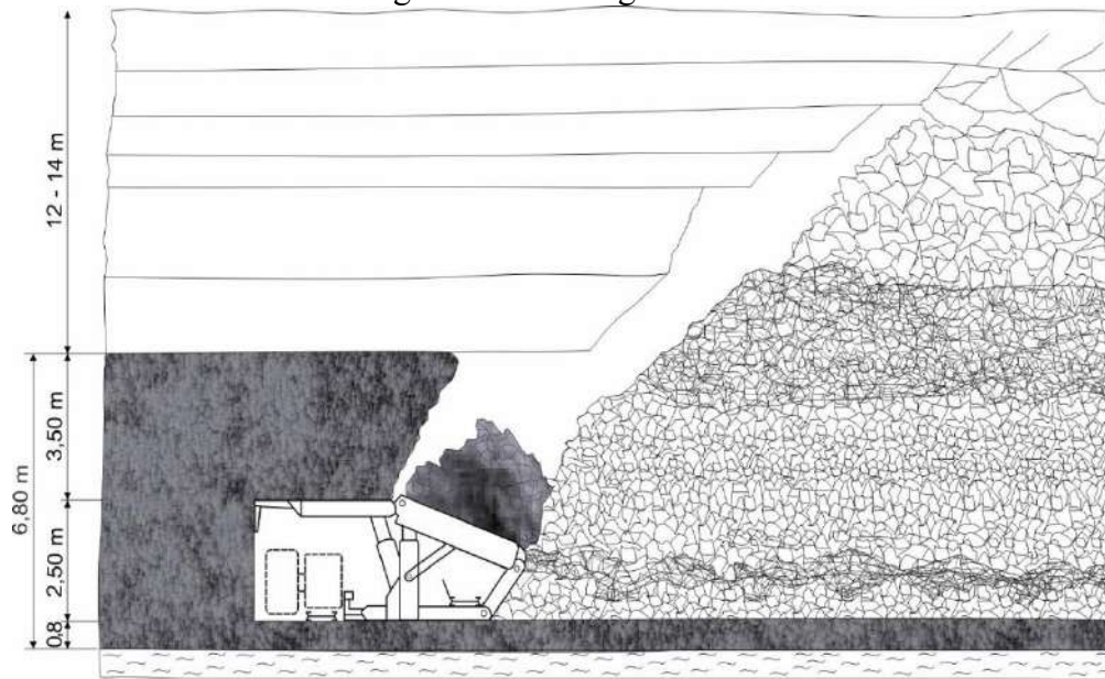
Figure 1. Total coal thickness mining of the Main coal seam in Raspočje mine using „Sublevel“ method with Dowty 4000 self-powered hydraulic support [8]
